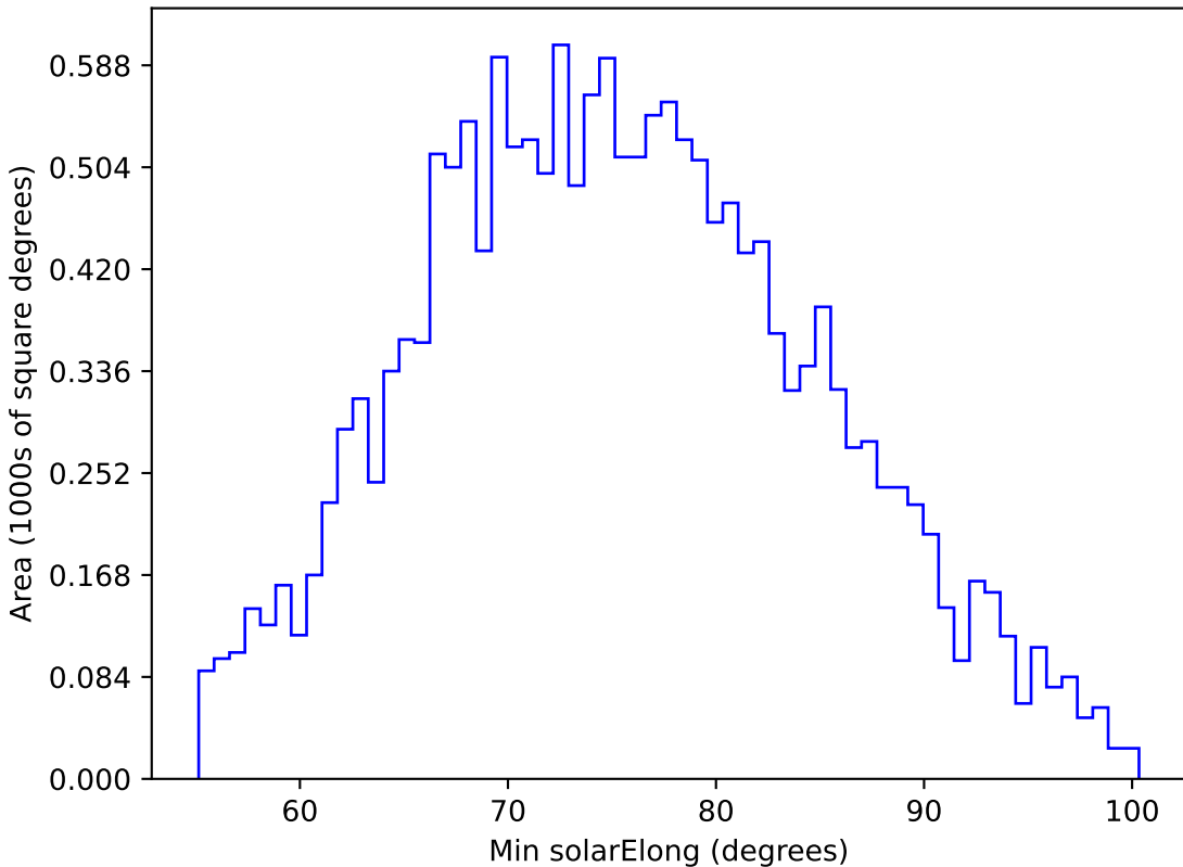
ddf_loaded_fl1_v3.4_10yrs WFD g band: Min solarElong
