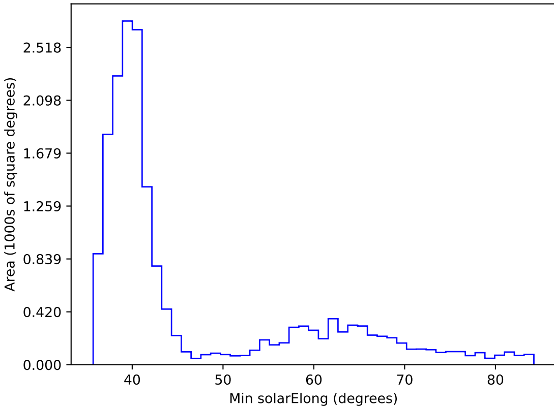
ddf_loaded_fl1_v3.4_10yrs WFD all bands: Min solarElong
