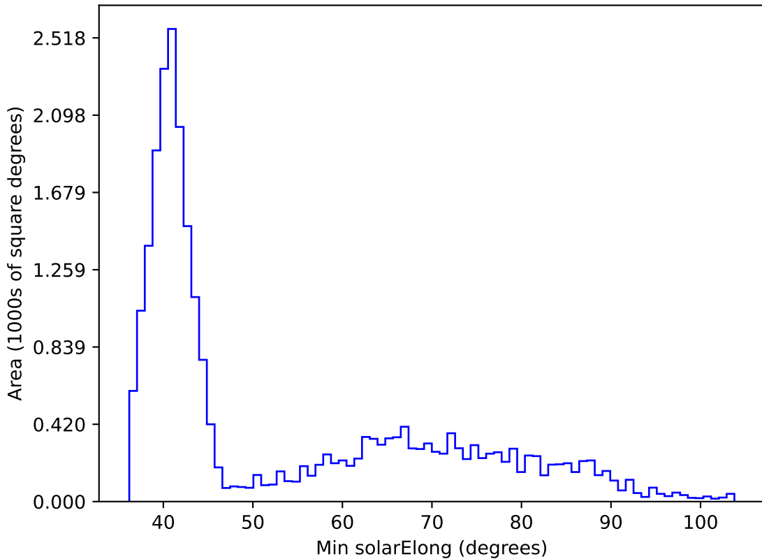
ddf_loaded_fl1_v3.4_10yrs All sky z band: Min solarElong
