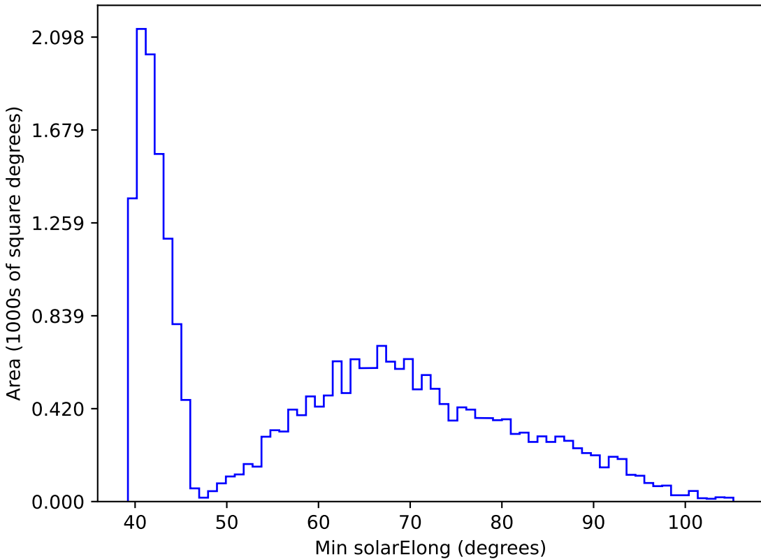
ddf_loaded_fl1_v3.4_10yrs All sky r band: Min solarElong
