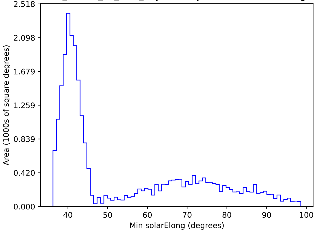
ddf_loaded_fl1_v3.4_10yrs All sky i band: Min solarElong
