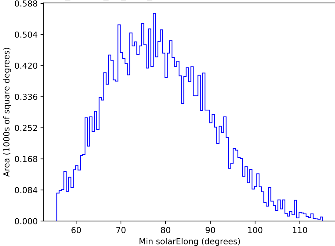
ddf_loaded_fl1_v3.4_10yrs All sky g band: Min solarElong
