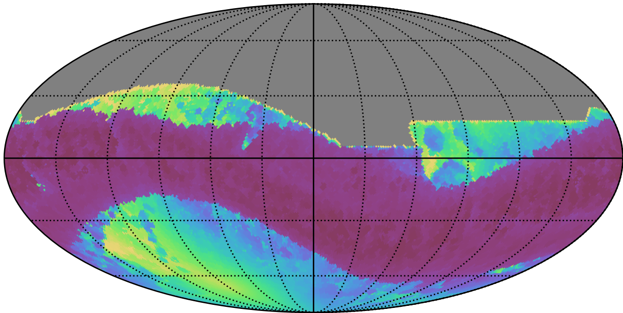
ddf_loaded_fl1_v3.4_10yrs All sky all bands: Min solarElong
