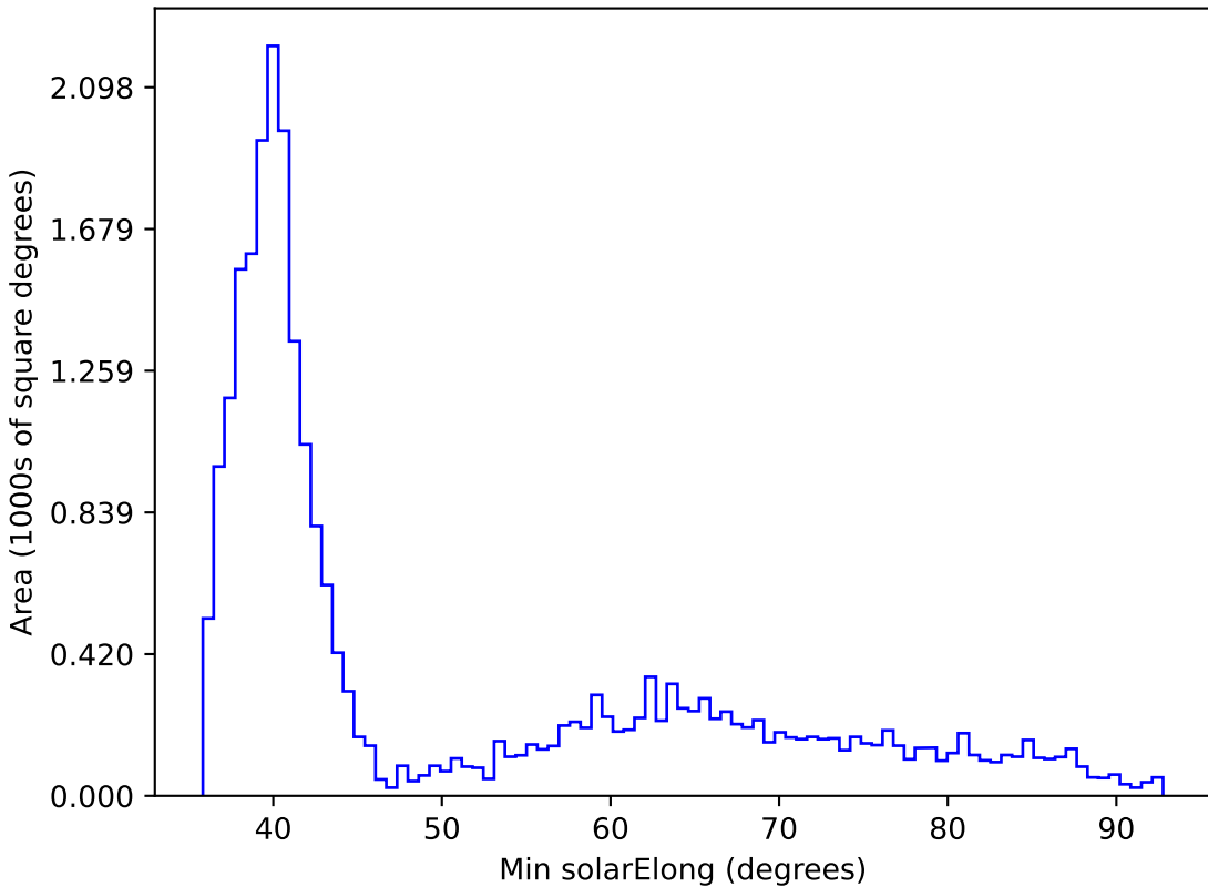
ddf_loaded_fl1_v3.4_10yrs All sky all bands: Min solarElong
