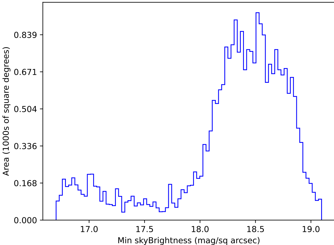
ddf_loaded_fl1_v3.4_10yrs Yr 1 z band: Min skyBrightness
