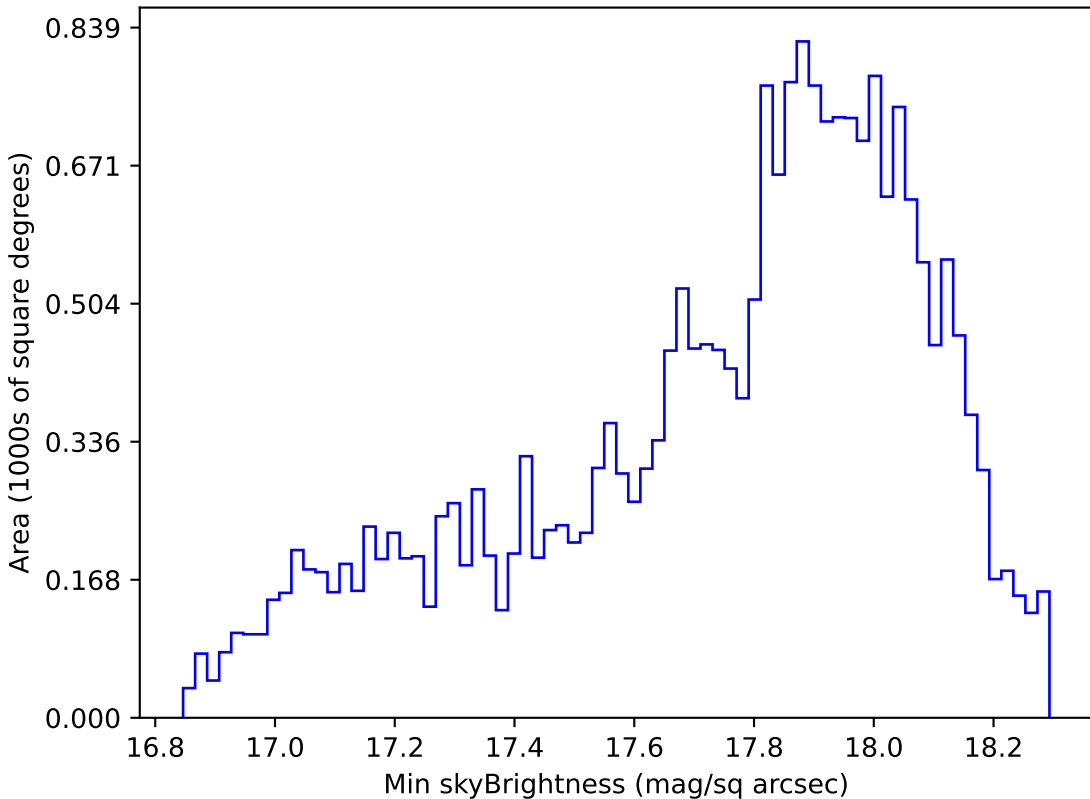
ddf_loaded_fl1_v3.4_10yrs Yr 1 y band: Min skyBrightness
