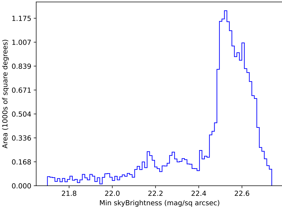
ddf_loaded_fl1_v3.4_10yrs Yr 1 u band: Min skyBrightness
