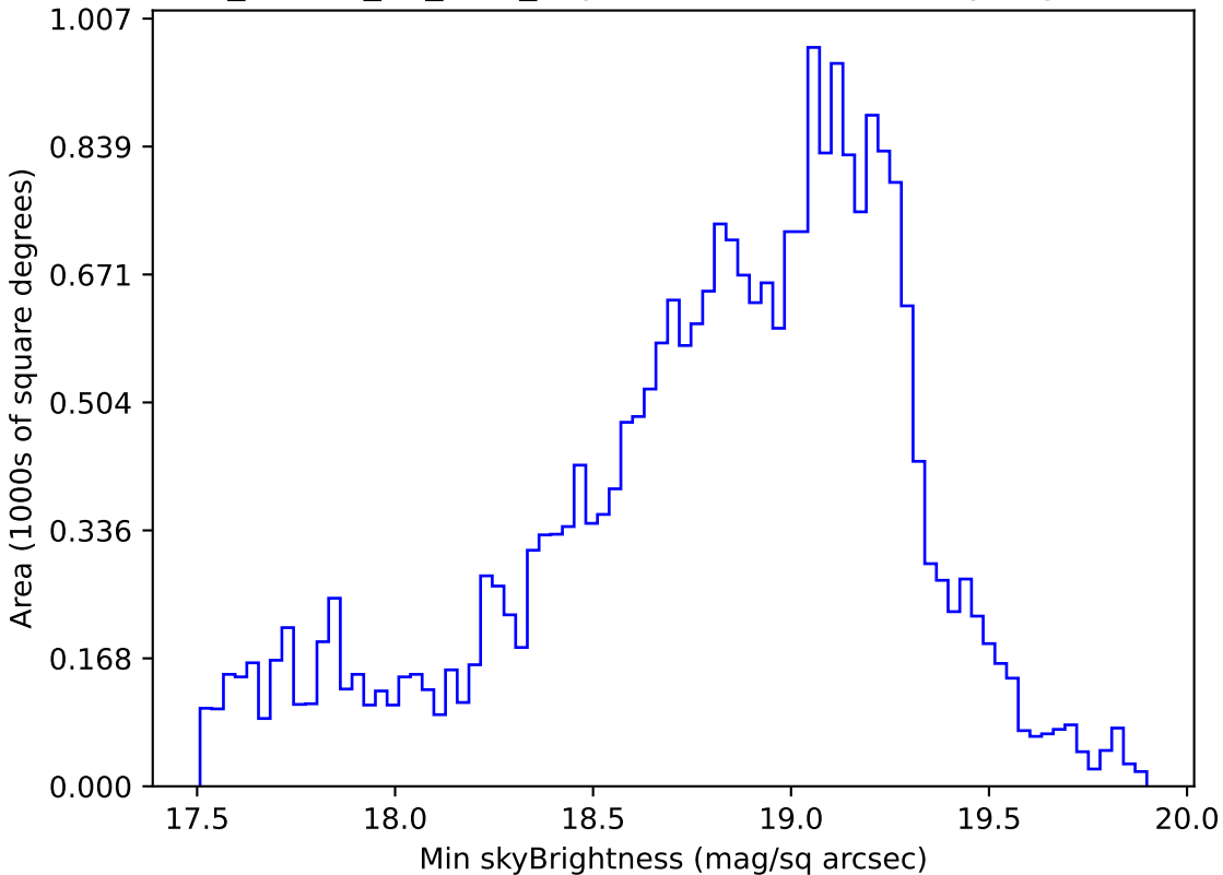
ddf_loaded_fl1_v3.4_10yrs Yr 1 i band: Min skyBrightness
