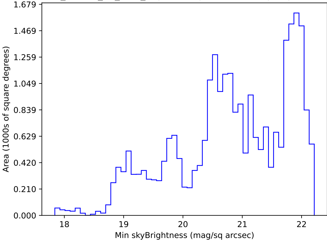
ddf_loaded_fl1_v3.4_10yrs Yr 1 g band: Min skyBrightness
