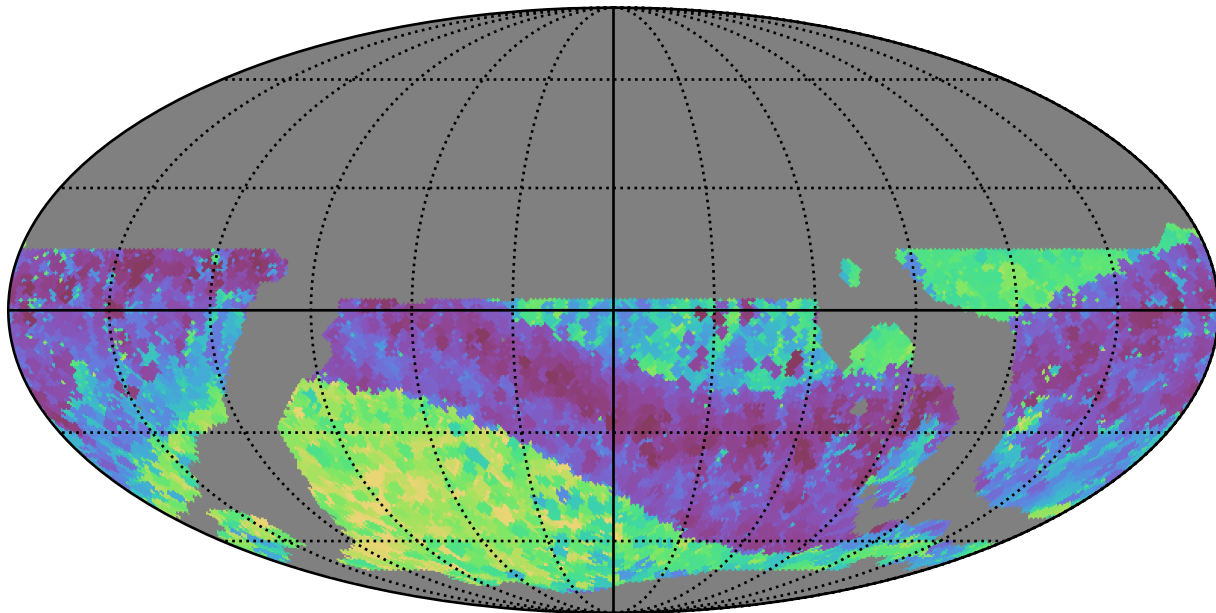
ddf_loaded_fl1_v3.4_10yrs WFD z band: Min skyBrightness
