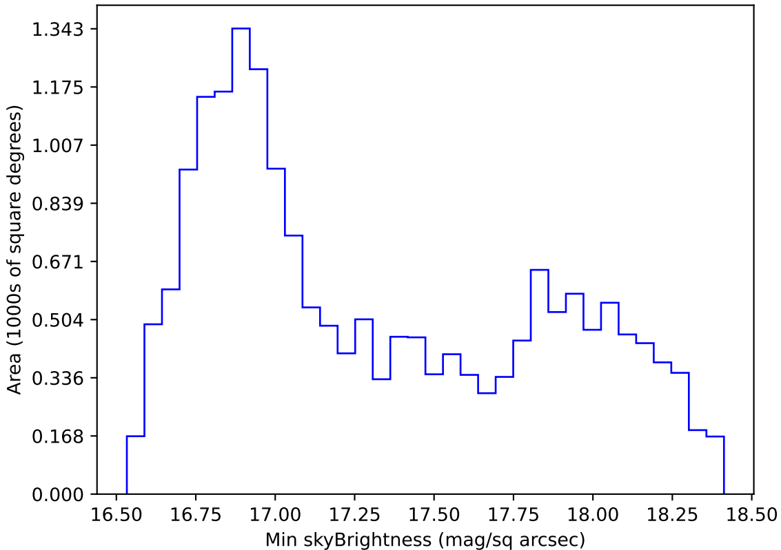
ddf_loaded_fl1_v3.4_10yrs WFD z band: Min skyBrightness
