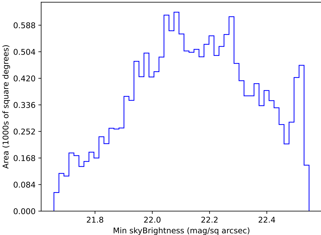
ddf_loaded_fl1_v3.4_10yrs WFD u band: Min skyBrightness
