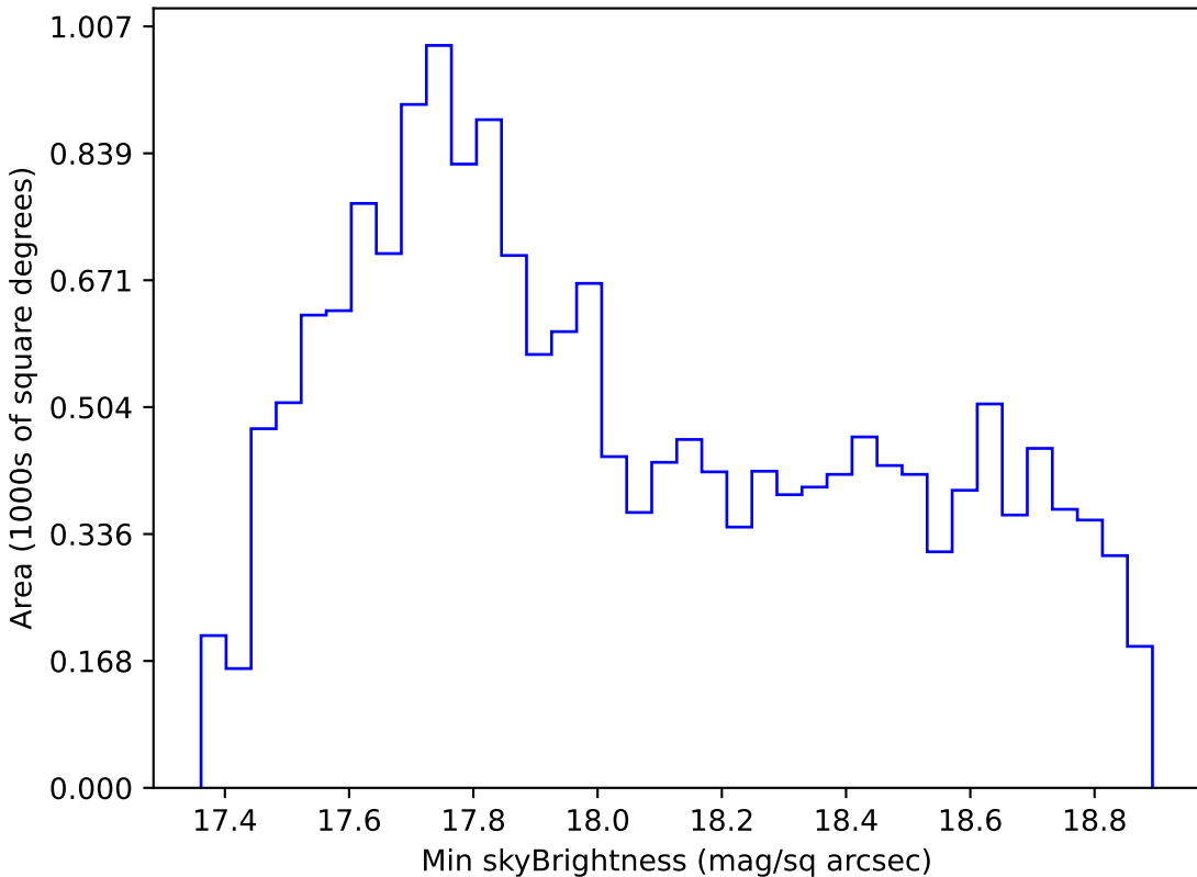
ddf_loaded_fl1_v3.4_10yrs WFD i band: Min skyBrightness
