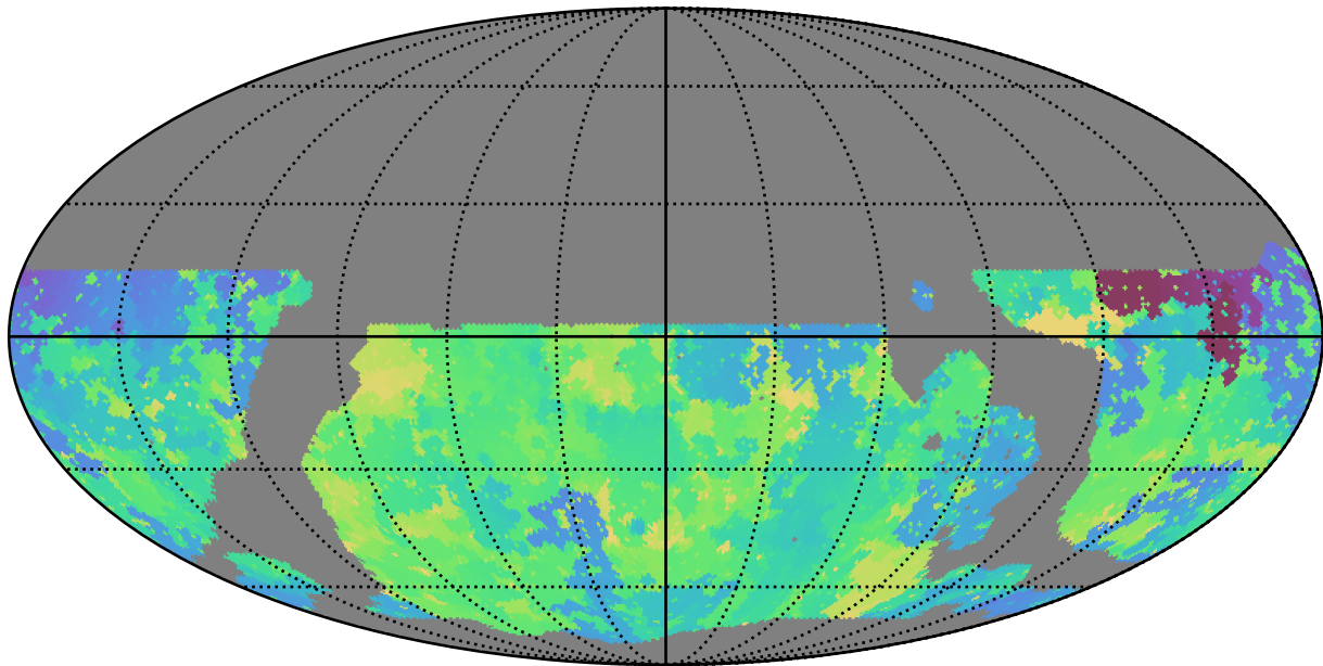
ddf_loaded_fl1_v3.4_10yrs WFD g band: Min skyBrightness
