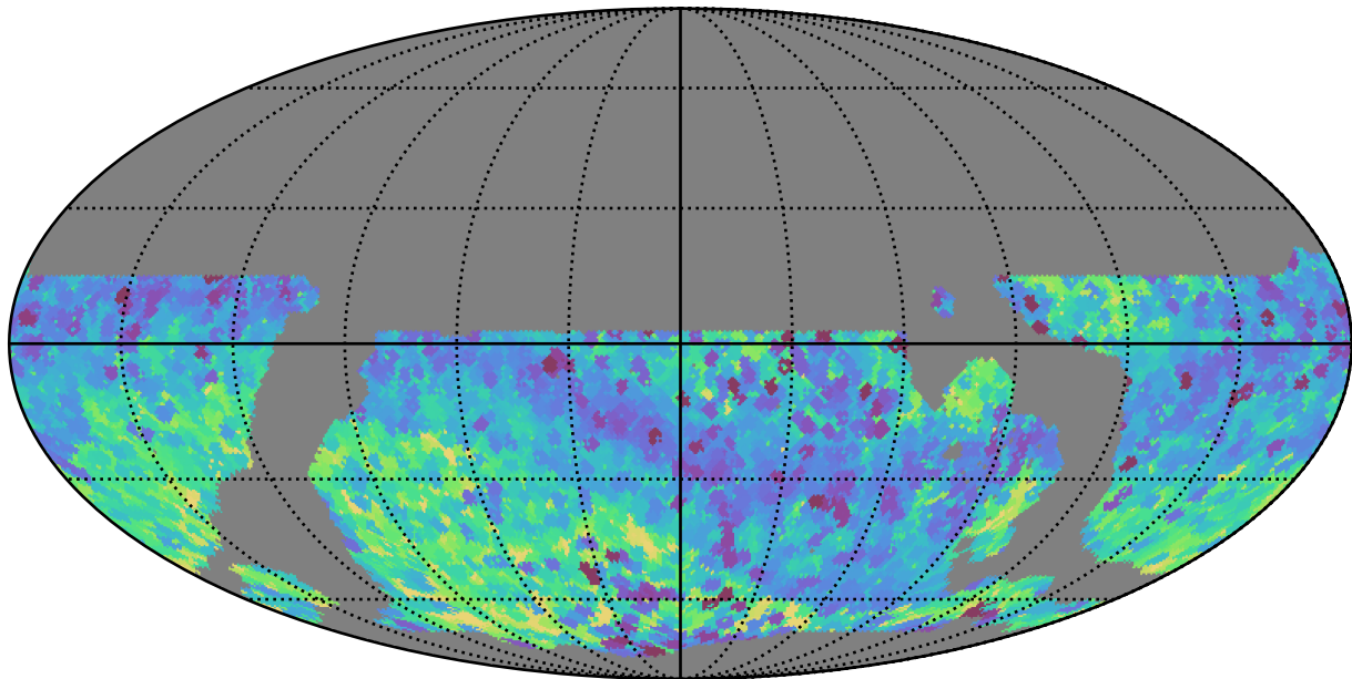
ddf_loaded_fl1_v3.4_10yrs WFD all bands: Min skyBrightness
