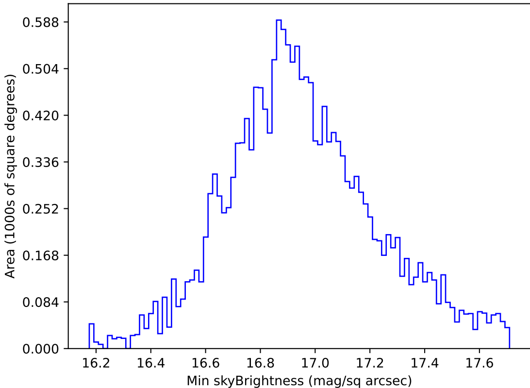
ddf_loaded_fl1_v3.4_10yrs WFD all bands: Min skyBrightness
