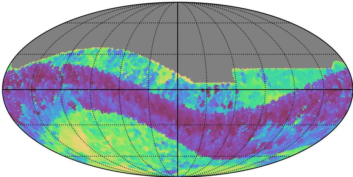
ddf_loaded_fl1_v3.4_10yrs All sky z band: Min skyBrightness
