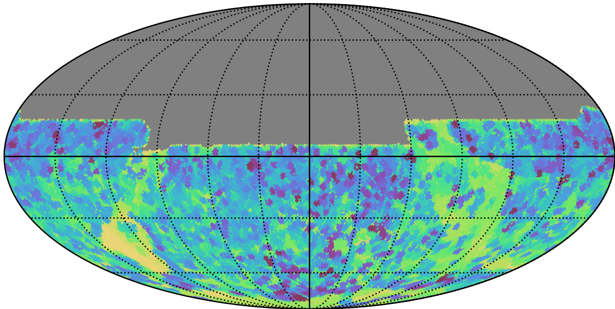
ddf_loaded_fl1_v3.4_10yrs All sky y band: Min skyBrightness
