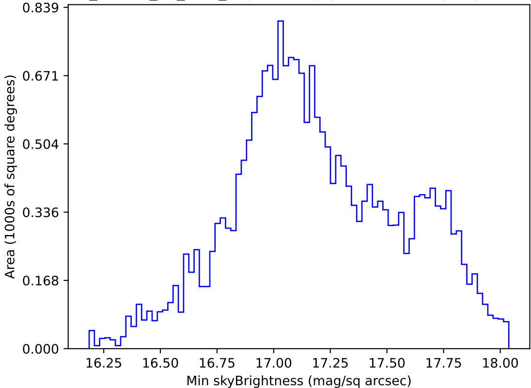
ddf_loaded_fl1_v3.4_10yrs All sky y band: Min skyBrightness
