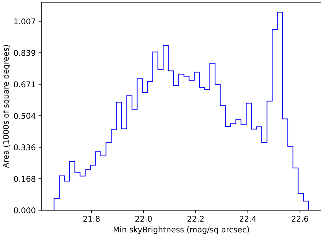
ddf_loaded_fl1_v3.4_10yrs All sky u band: Min skyBrightness
