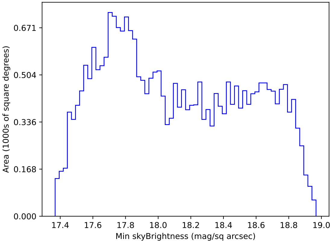
ddf_loaded_fl1_v3.4_10yrs All sky i band: Min skyBrightness
