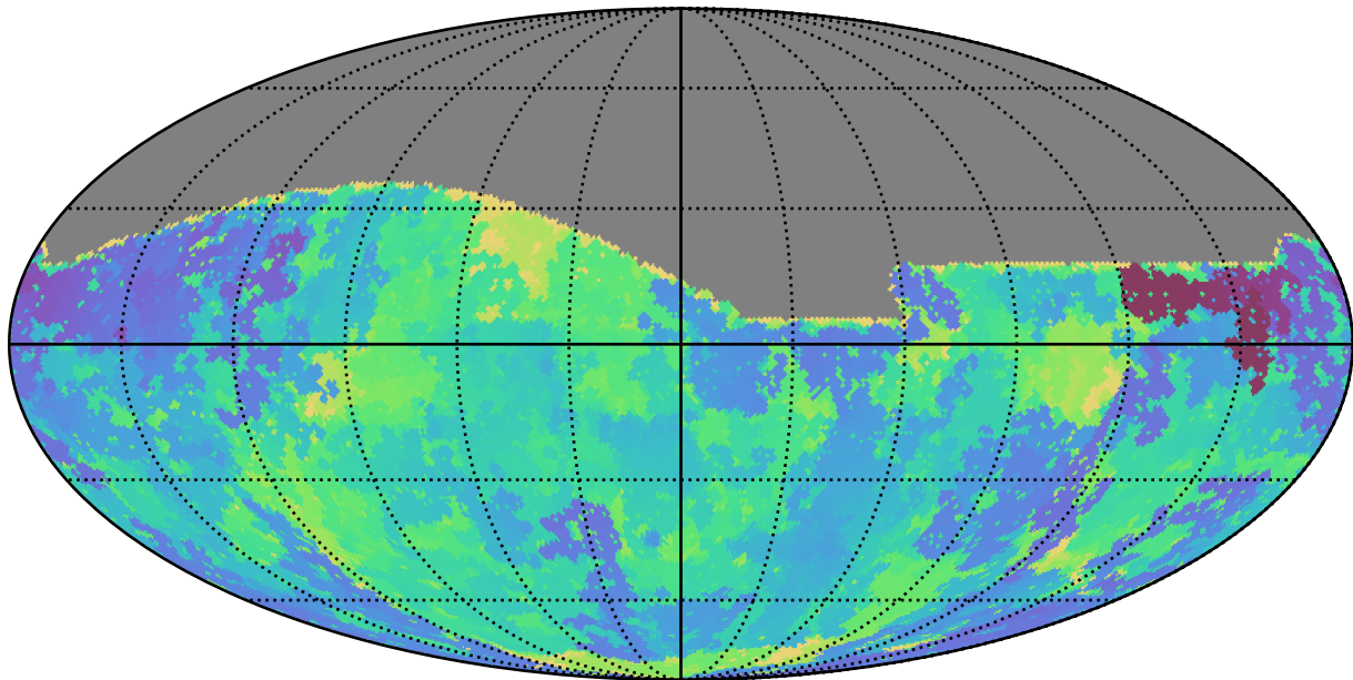
ddf_loaded_fl1_v3.4_10yrs All sky g band: Min skyBrightness
