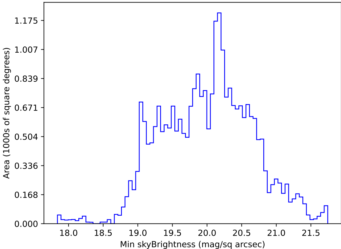
ddf_loaded_fl1_v3.4_10yrs All sky g band: Min skyBrightness
