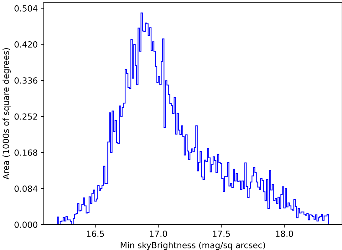
ddf_loaded_fl1_v3.4_10yrs All sky all bands: Min skyBrightness
