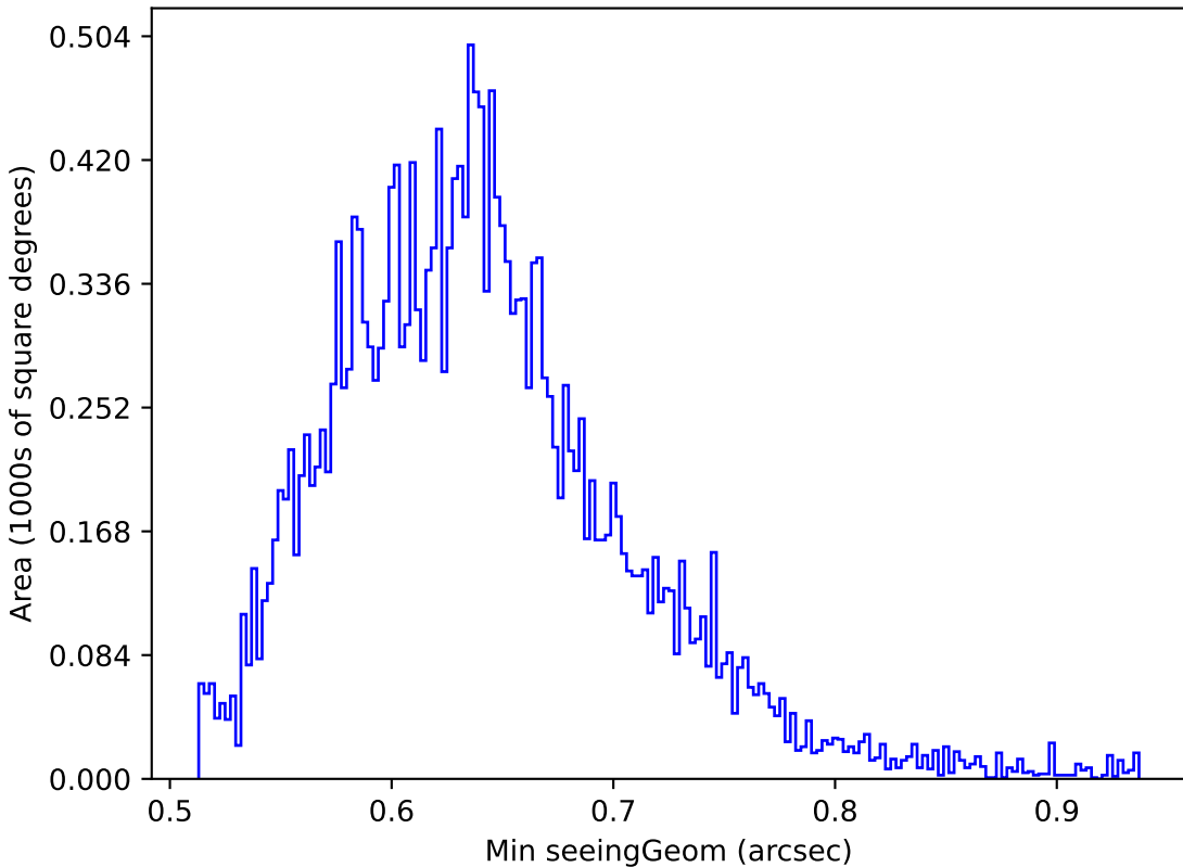
ddf_loaded_fl1_v3.4_10yrs Yr 1 y band: Min seeingGeom
