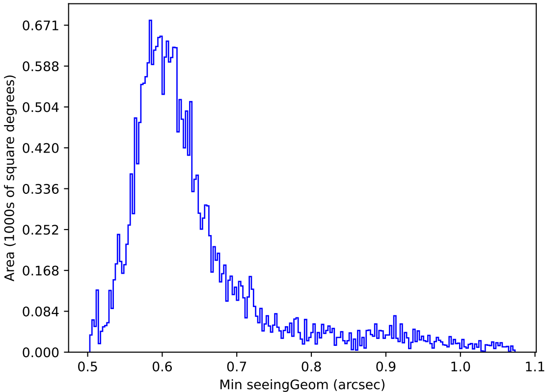
ddf_loaded_fl1_v3.4_10yrs Yr 1 r band: Min seeingGeom
