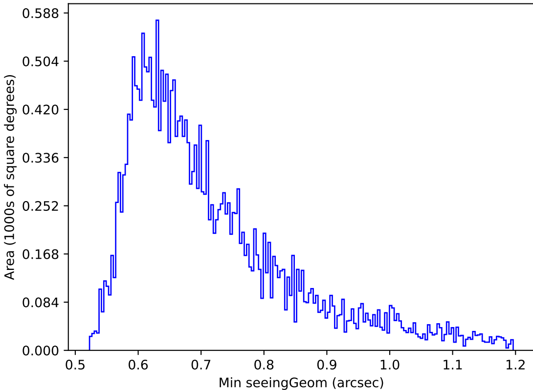
ddf_loaded_fl1_v3.4_10yrs Yr 1 g band: Min seeingGeom
