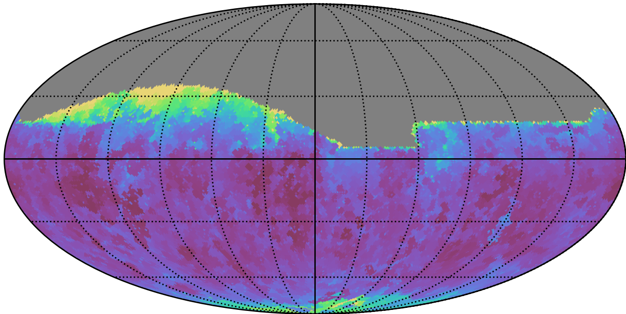
ddf_loaded_fl1_v3.4_10yrs Yr 1 all bands: Min seeingGeom
