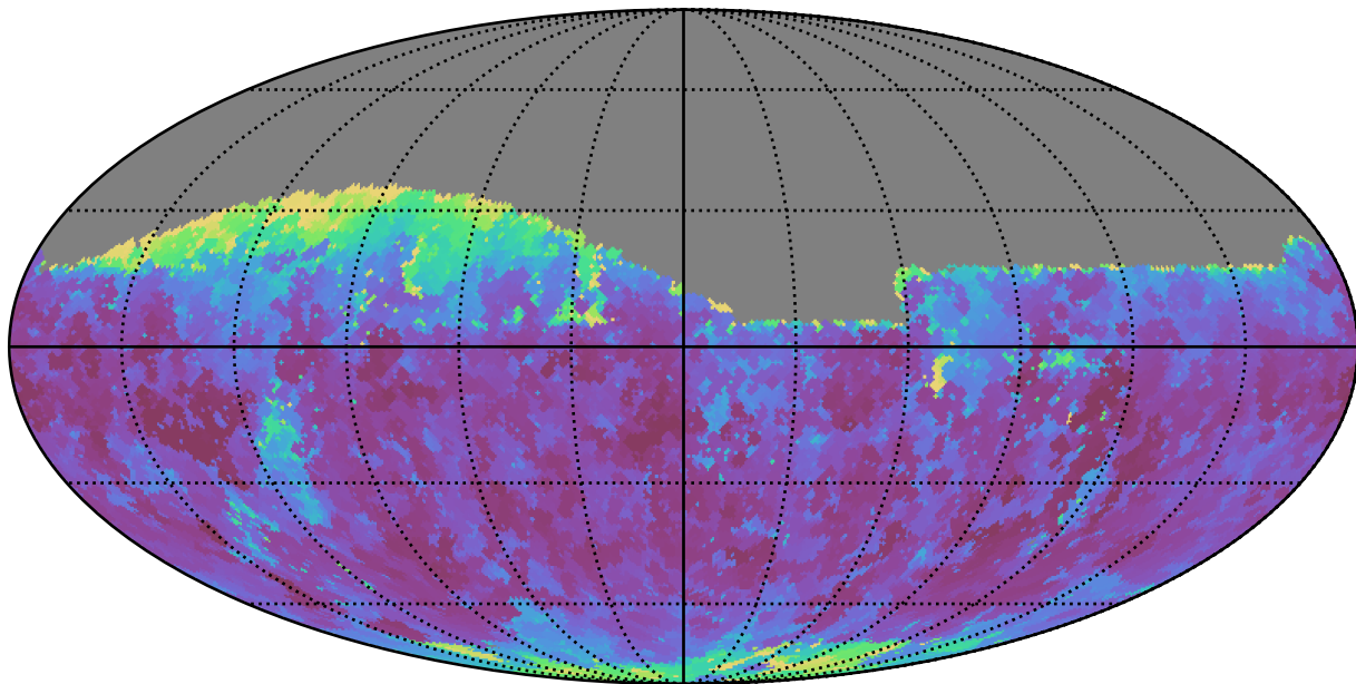
ddf_loaded_fl1_v3.4_10yrs Yr 1 z band: Min seeingEff
