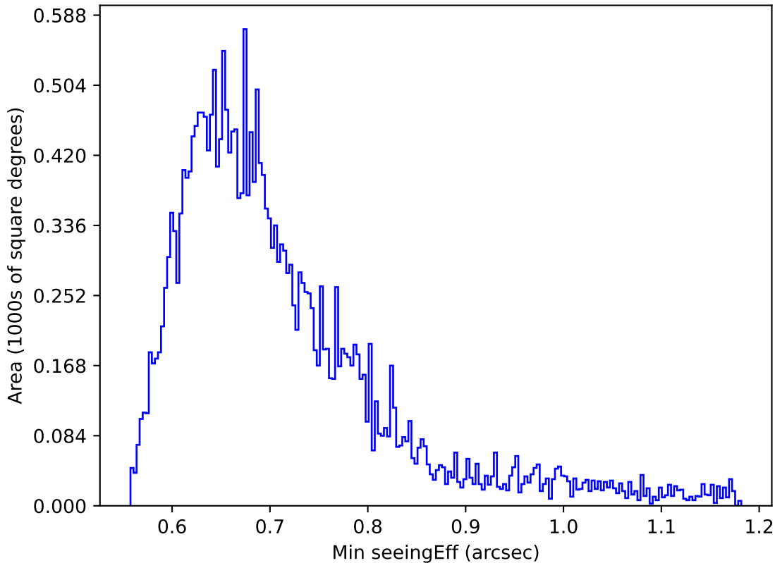
ddf_loaded_fl1_v3.4_10yrs Yr 1 z band: Min seeingEff
