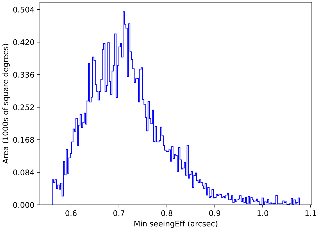
ddf_loaded_fl1_v3.4_10yrs Yr 1 y band: Min seeingEff
