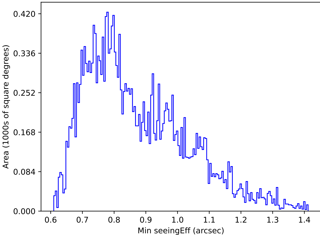
ddf_loaded_fl1_v3.4_10yrs Yr 1 u band: Min seeingEff
