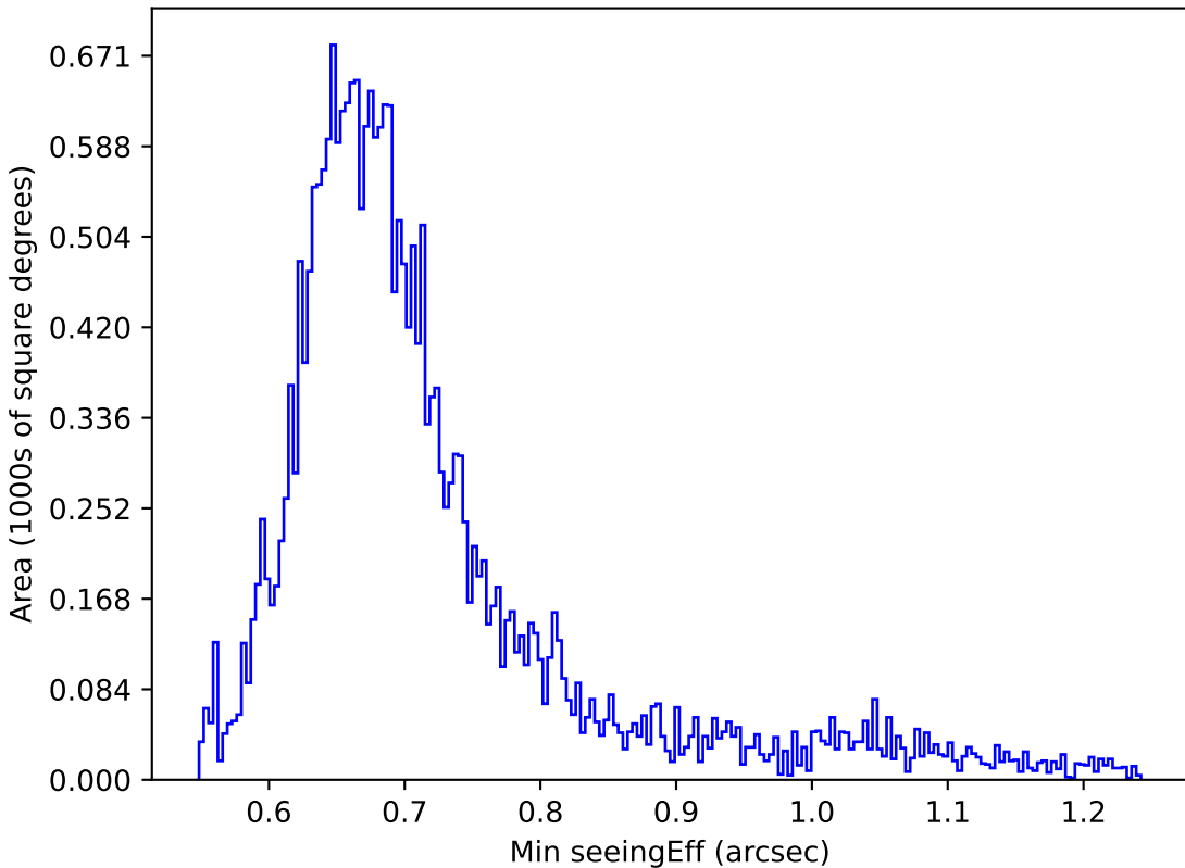
ddf_loaded_fl1_v3.4_10yrs Yr 1 r band: Min seeingEff
