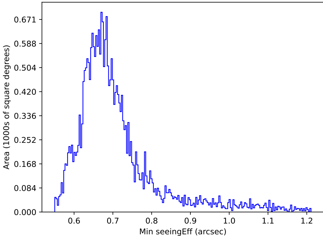
ddf_loaded_fl1_v3.4_10yrs Yr 1 i band: Min seeingEff
