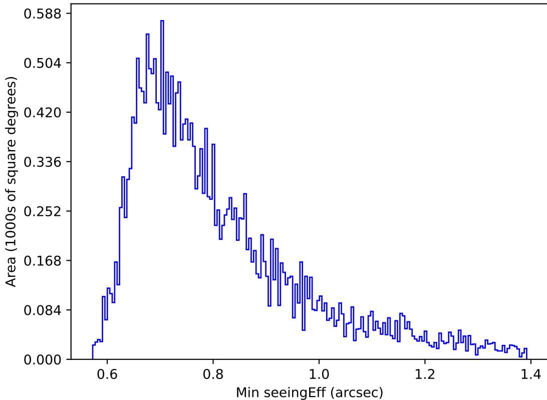
ddf_loaded_fl1_v3.4_10yrs Yr 1 g band: Min seeingEff
