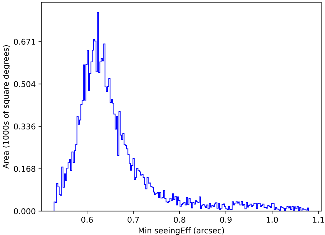
ddf_loaded_fl1_v3.4_10yrs Yr 1 all bands: Min seeingEff
