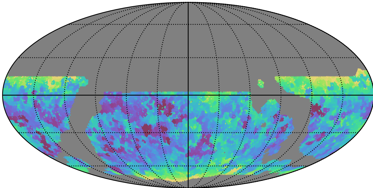
ddf_loaded_fl1_v3.4_10yrs WFD z band: Min seeingEff
