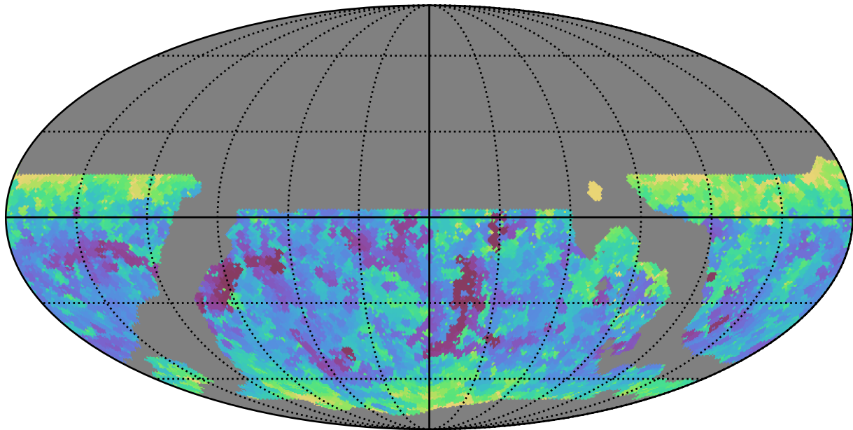
ddf_loaded_fl1_v3.4_10yrs WFD y band: Min seeingEff
