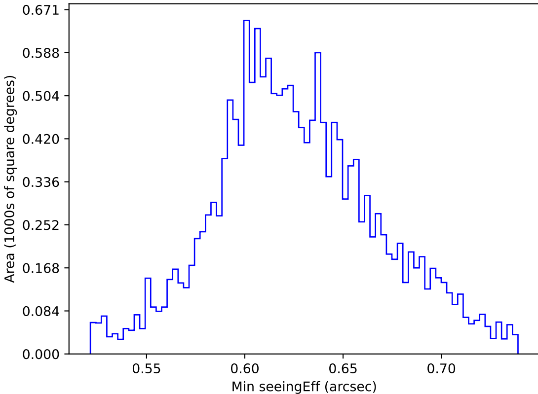
ddf_loaded_fl1_v3.4_10yrs WFD y band: Min seeingEff
