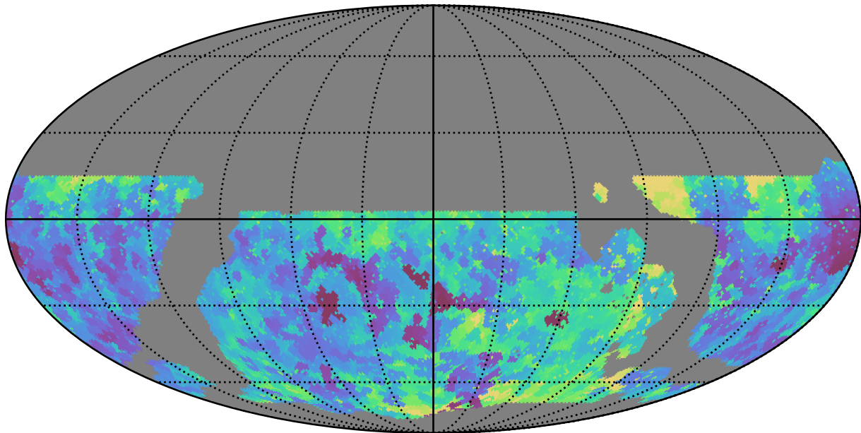
ddf_loaded_fl1_v3.4_10yrs WFD u band: Min seeingEff
