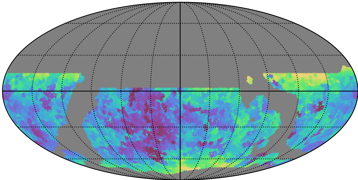
ddf_loaded_fl1_v3.4_10yrs WFD r band: Min seeingEff
