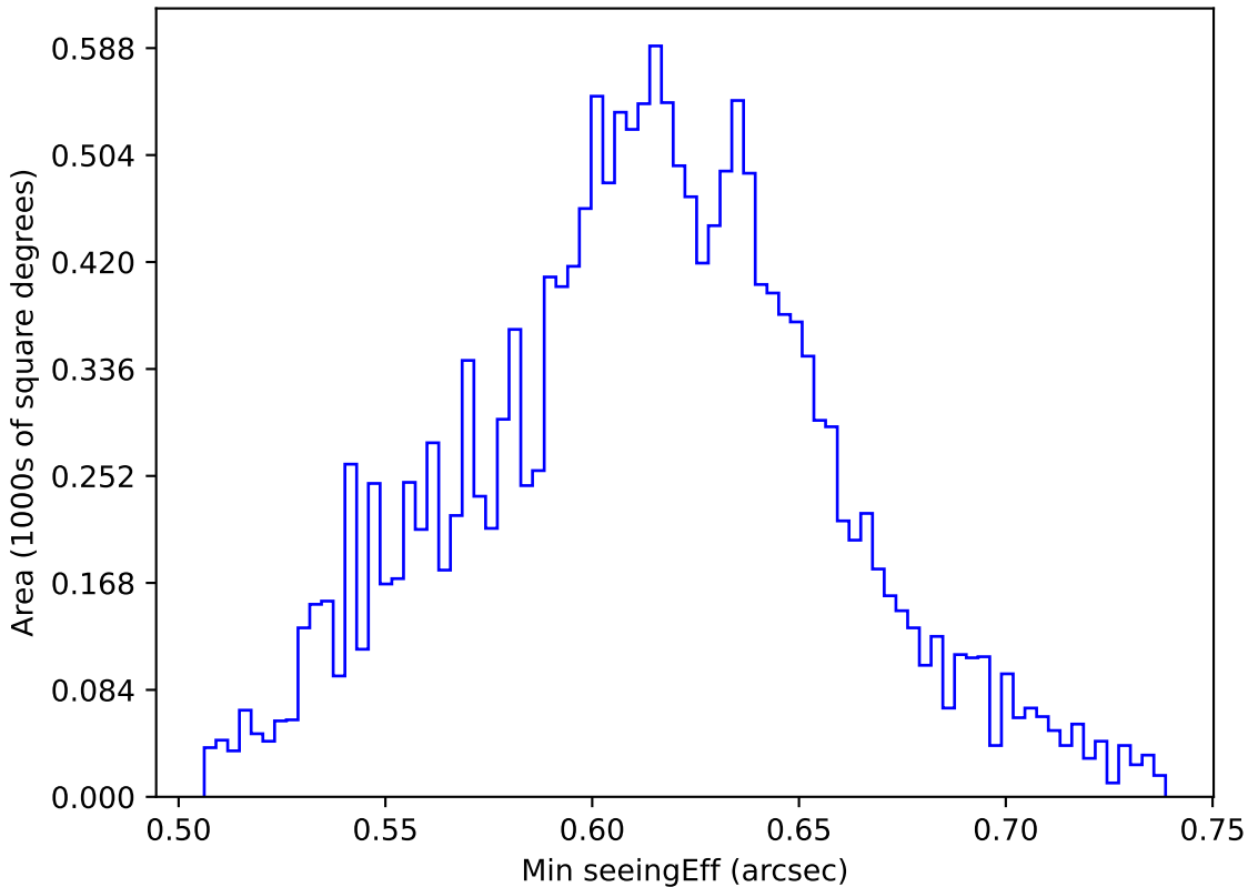
ddf_loaded_fl1_v3.4_10yrs WFD r band: Min seeingEff
