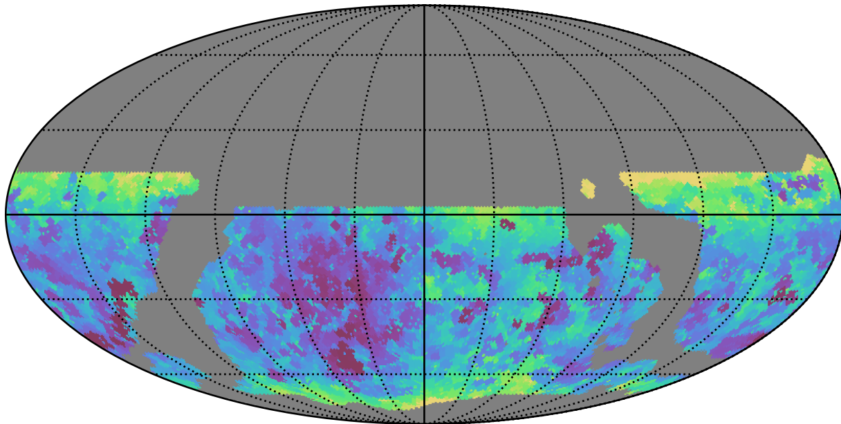
ddf_loaded_fl1_v3.4_10yrs WFD i band: Min seeingEff
