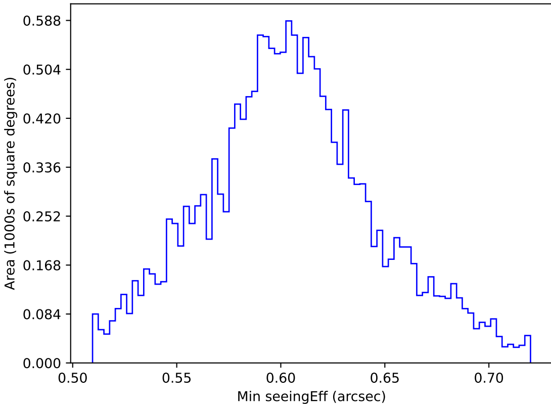
ddf_loaded_fl1_v3.4_10yrs WFD i band: Min seeingEff
