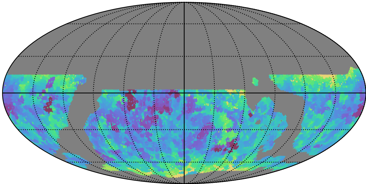
ddf_loaded_fl1_v3.4_10yrs WFD g band: Min seeingEff
