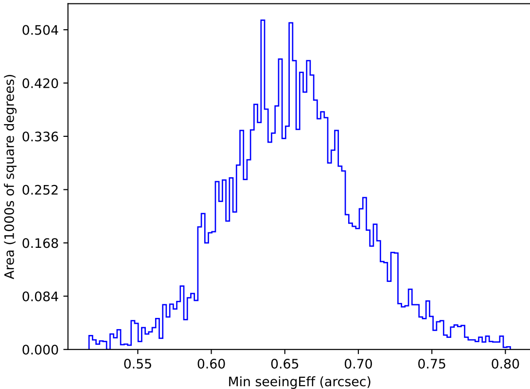
ddf_loaded_fl1_v3.4_10yrs WFD g band: Min seeingEff
